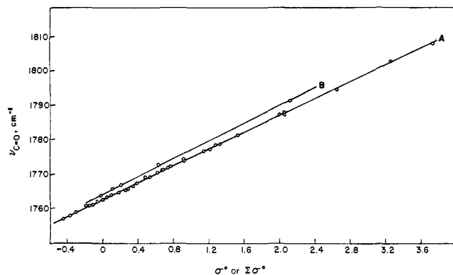
Figure 1. Correlations of carbonyl-stretching frequency for substituted phenyl hydrocinnamates (in carbon tetrachloride) with \sigma^0 or \Sigma\sigma^0 for phenyl substituents: (A) correlation for 48 compounds obeying eq 1; (B) correlation for five compounds (containing o -F or o -OCH 3 groups) obeying eq 2.
